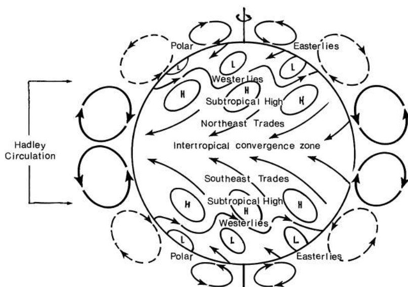
Schematic diagram of the general atmospheric circulation.
