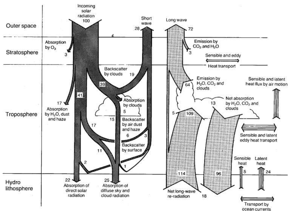
Schematic diagram showing the interactions that radiation undergoes in the atmosphere. Source: Lockwood (1979).
