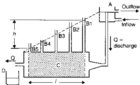
Darcy's law. Apparatus showing the relationships expressed in Darcy's law: A, constant-head device; B, manometers; C, porous medium being measured; D, outflow with discharge Q . Note the change in head h with distance l .
