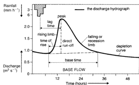
Storm hydrograph.
