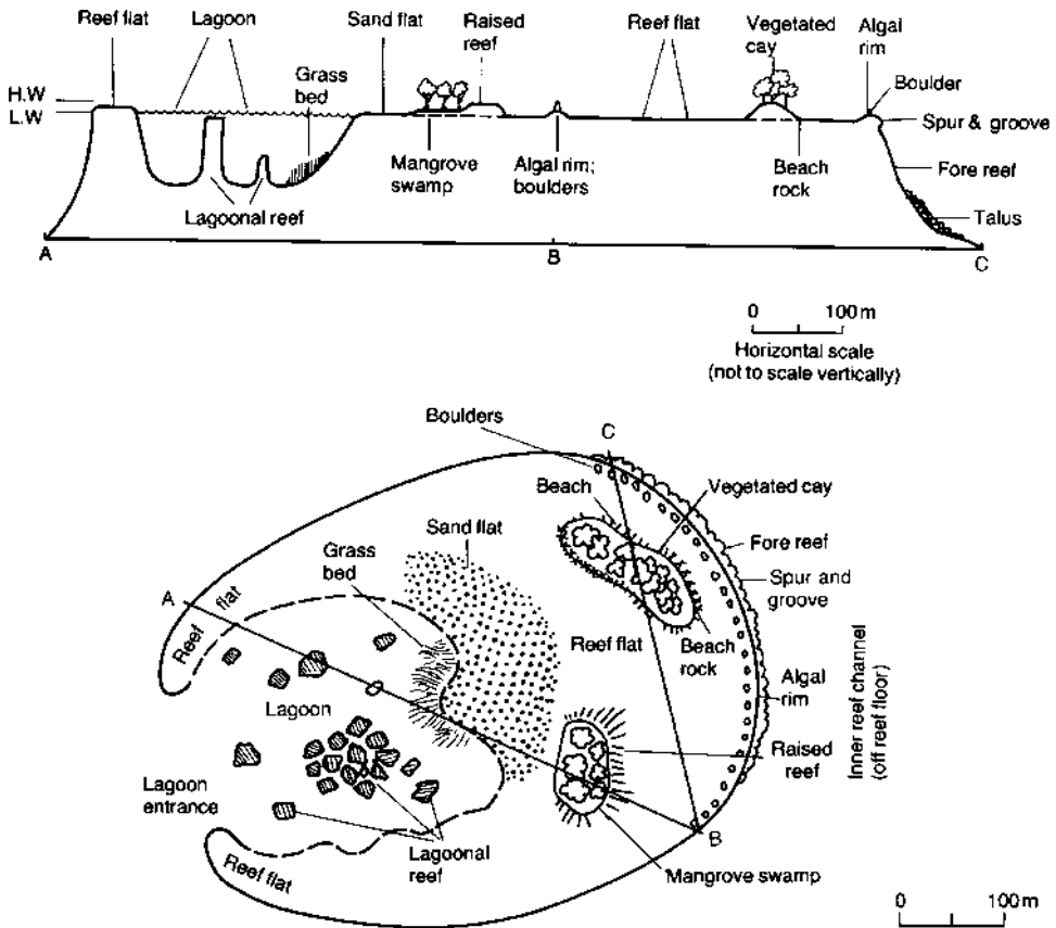
Coral-algal reefs. Plan and cross-section of an ideal coral reef, showing the major environments.
