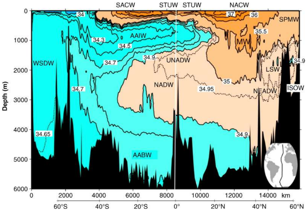
NADW meridional salinity transect at 20–25°W for the Atlantic Ocean showing the extent of NADW and the main water masses that form NADW. UNADW: Upper NADW; LSW: Labrador Sea Water; SPMW: Subpolar Mode Water; MW: Mediterranean Water; ISOW: Iceland–Scotland Overflow Water; AAIW: Antarctic Intermediate Water; AABW: Antarctic Bottom Water.
