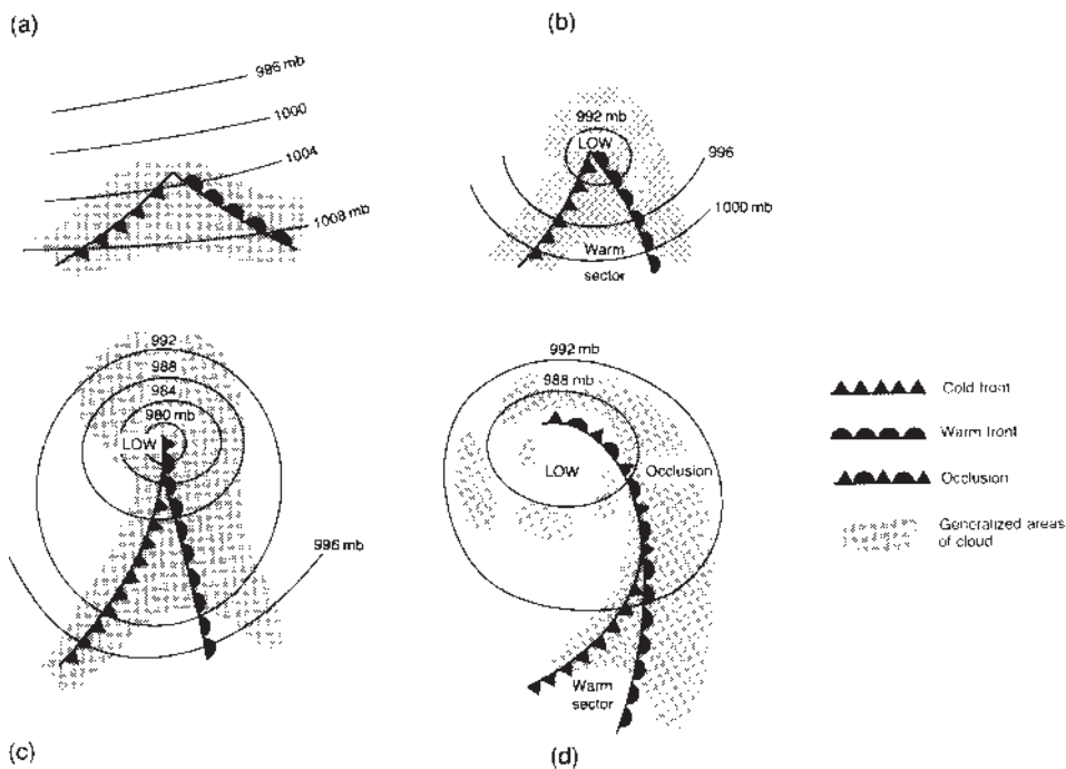
Extratropical cyclone.
