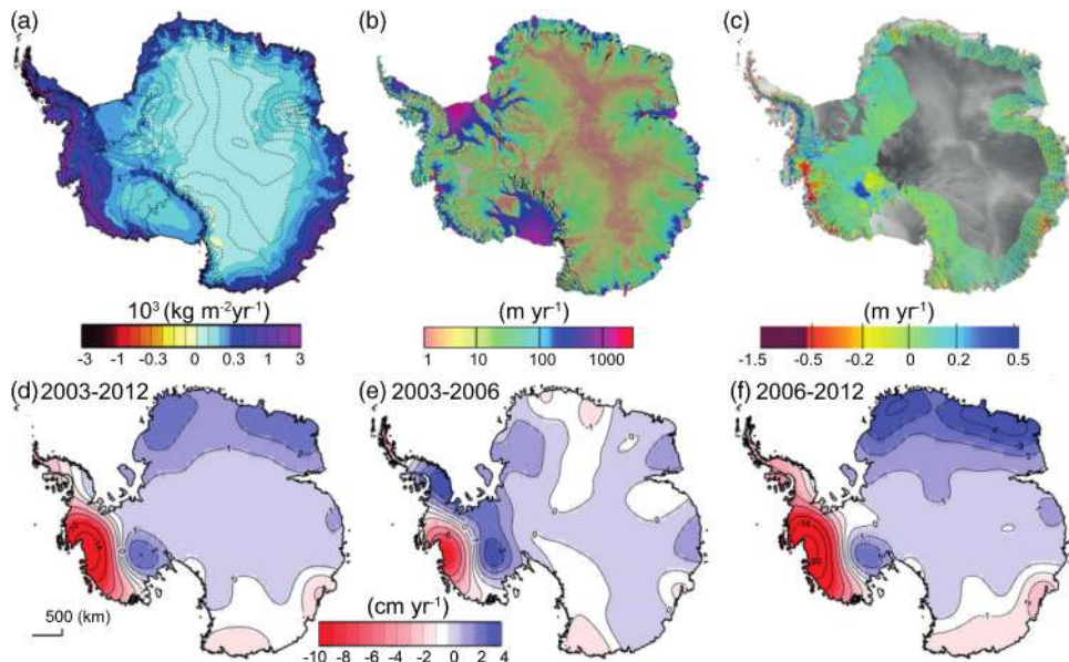
Antarctic ice sheet: (a) mean surface mass balance for 1989–2004 from regional atmospheric modelling; (b) ice sheet velocity for 2007–2009 determined from satellite data; (c) changes in ice sheet surface elevation for 2003–2008 determined from ICESat altimetry; temporal evolution of ice loss determined from GRACE for time periods (d) 2003–2012, (e) 2003–2006 and (f) 2006–2012.
