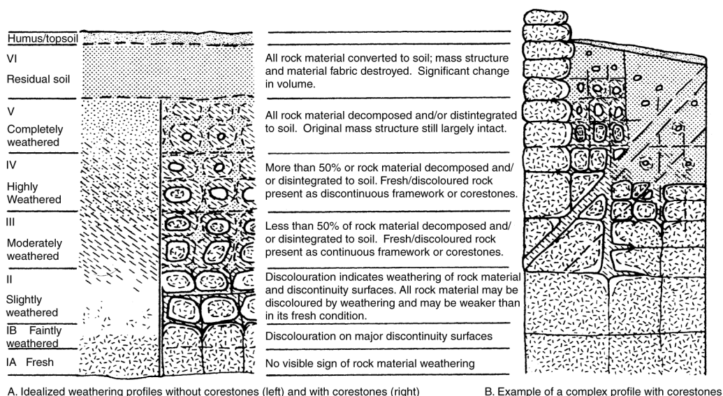
A. Idealized weathering profiles without corestones (left) and with corestones (right)
