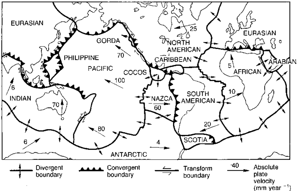
Plate tectonics. Map of the lithospheric plates. The various types of plate boundary are shown and the estimated current rates ( \text{mm a}^{-1} ) and directions of plate movements are indicated.
