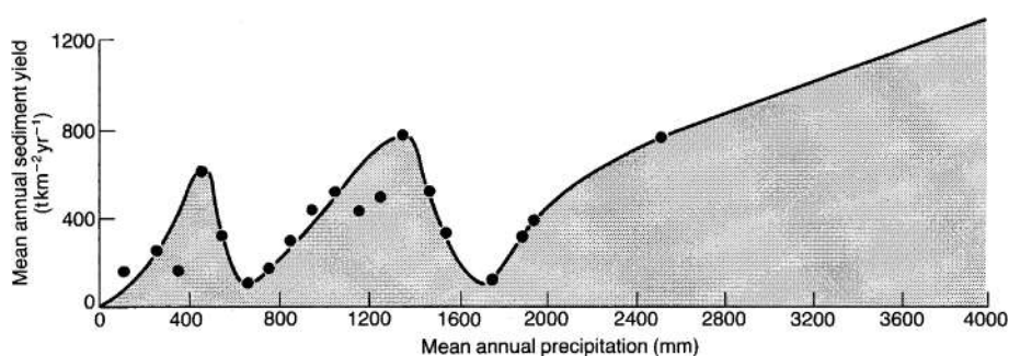
Sediment yield. The relationship between mean annual sediment yield and mean annual precipitation.
