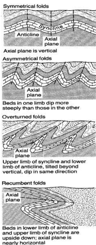
Fold 2: diagrammatic illustration of symmetrical, asymmetrical, overturned and recumbent folds.
