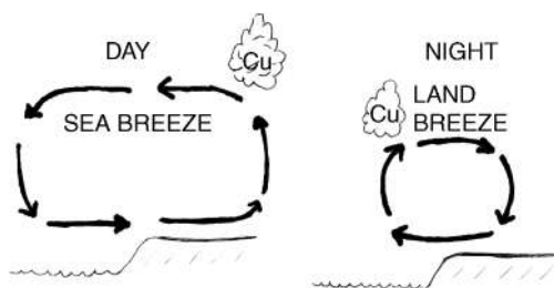
Schematic diagram of a sea breeze and a land breeze.
