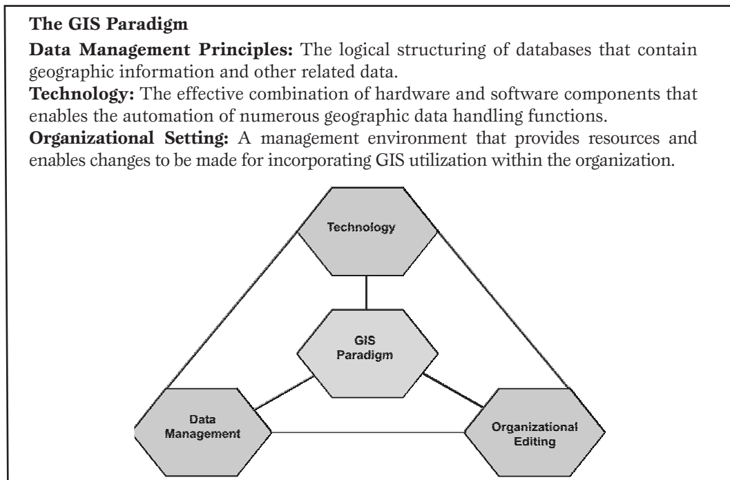
Figure 12.2: GIS paradigm.
